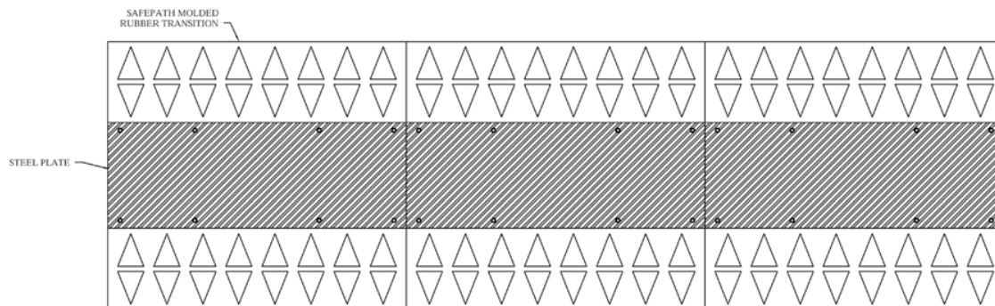
Seismic Transition Cover – Top View
